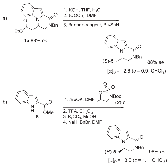
Scheme 3. Determination of the absolute configuration of product 1a . THF: tetrahydrofuran; DMF: N,N -dimethylformamide; Boc: tert -butoxycarbonyl; TFA: trifluoroacetic acid.
