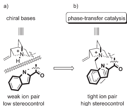
Figure 1. Chiral organic bases versus phase-transfer catalysis in the enantioselective ring closure of 3 .
